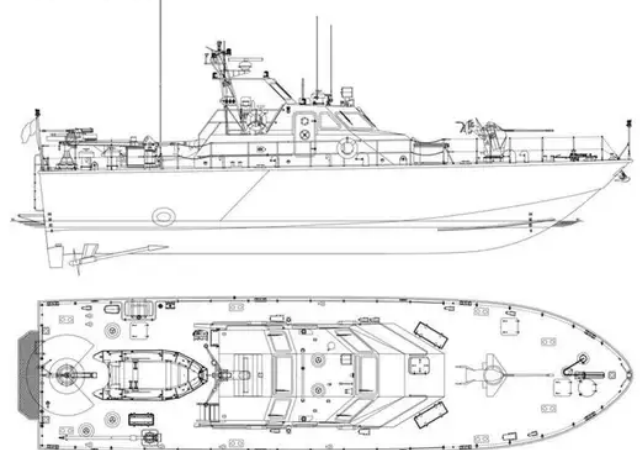
M21 PATROL BOAT
